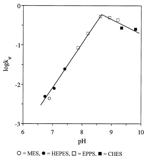
Figure 4. pH Dependence of the rate constant for the cleavage of \beta -AlaPNP in 1:1 DMSO/water by \text{Cu}^{\text{II}} -saturated polymer 2 ( n = 10 ). Symbols indicate the different buffers used; for buffer abbreviations see the Experimental Section
