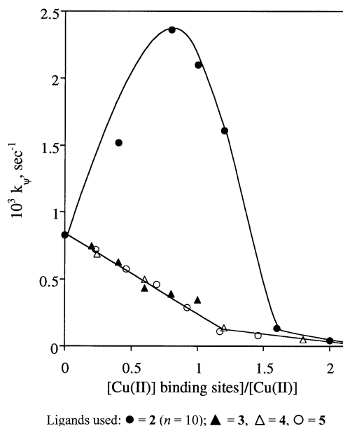
Figure 3. Dependence of the observed rate constant, k_{\text{p}} , for the cleavage of \beta -AlaPNP from the binding sites (i.e. the number of pyridine subunits) over \text{Cu}^{\text{II}} concentrations ratio in 1:1 DMSO/water at pH 6.3. [\text{Cu}^{\text{II}}] is constant = 5 \cdot 10^{-4} \text{ M}
