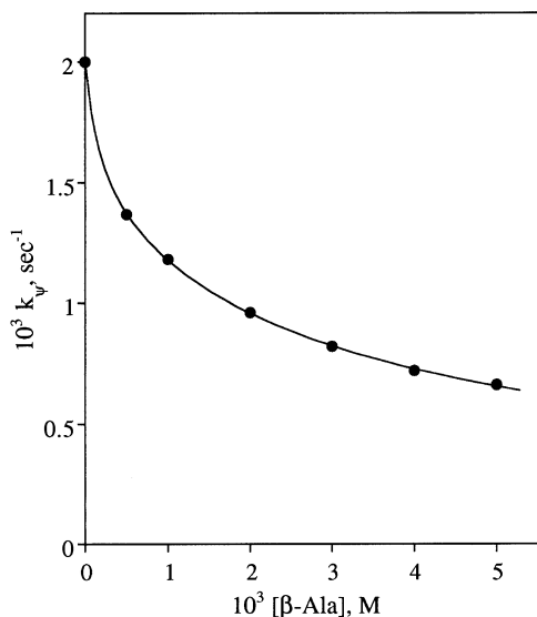
Figure 6. Dependence of the observed rate constant, k_{\text{p}} , for the cleavage of \beta -AlaPNP from the concentration of added \beta -alanine ( \beta -Ala) in the presence of \text{Cu}^{\text{II}} -loaded polymer 2 ( n = 10 ). Conditions: 1:1 DMSO/water, pH = 6.3, 25°C, [\text{Cu}^{\text{II}}] = 4 \cdot 10^{-4} \text{ M}
