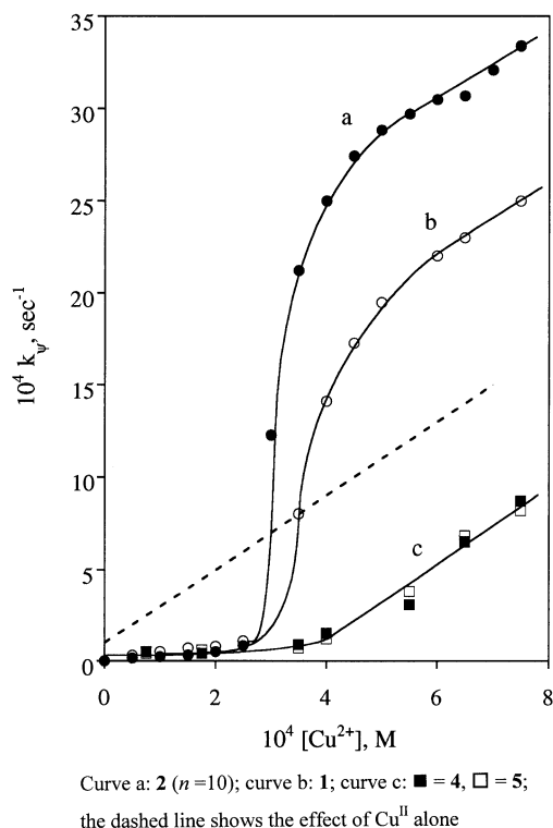
Figure 2. Dependence of the observed rate constant, k_{\text{p}} , for the cleavage of \beta -AlaPNP from the concentration of \text{Cu}^{\text{II}} in the presence of different ligands in 1:1 DMSO/water at pH 6.3. [Ligand's pyridine subunits] = 4 \cdot 10^{-4} \text{ M}
