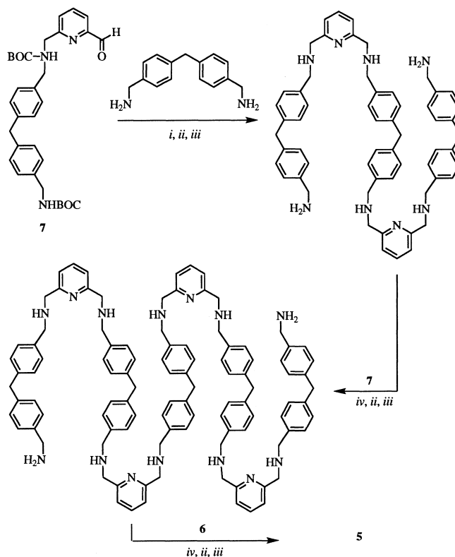
Scheme 2. Synthetic route to oligomer 5 . Reagents: i) \text{CH}_2\text{Cl}_2 , molecular sieves; ii) \text{NaBH}_4 , \text{EtOH}/\text{CH}_2\text{Cl}_2 ; iii) \text{CF}_3\text{COOH}/\text{CH}_2\text{Cl}_2 ; iv) Benzene, reflux
