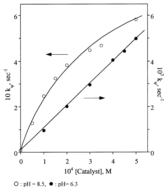
Figure 5. Dependence of the observed rate constant, k_v , for the cleavage of \beta -AlaPNP from the concentration of the \text{Cu}^{\text{II}} -saturated polymer 2 (catalyst) in 1:1 DMSO/water
