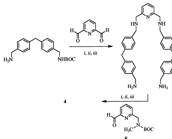
Scheme 1. Synthetic route to oligomer 4 . Reagents: i) Benzene, reflux; ii) \text{NaBH}_4 , \text{EtOH}/\text{CH}_2\text{Cl}_2 ; iii) \text{CF}_3\text{COOH}/\text{CH}_2\text{Cl}_2 ; \text{Na}_2\text{CO}_3 10%
