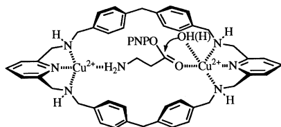
Figure 1. Suggested mechanism for the cleavage of \beta -AlaPNP by the dinuclear complex 1 \cdot 2 \text{ Cu}^{\text{II}}
